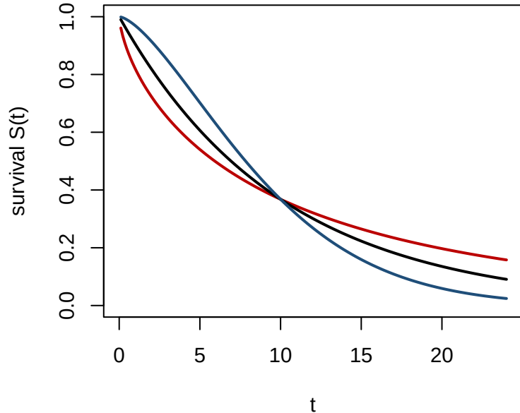
Implied survival
