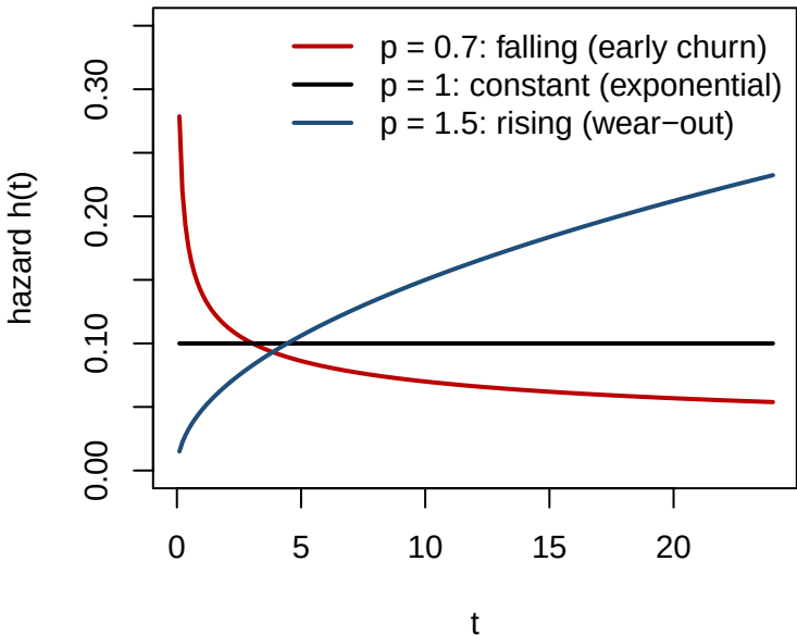
Weibull hazards
